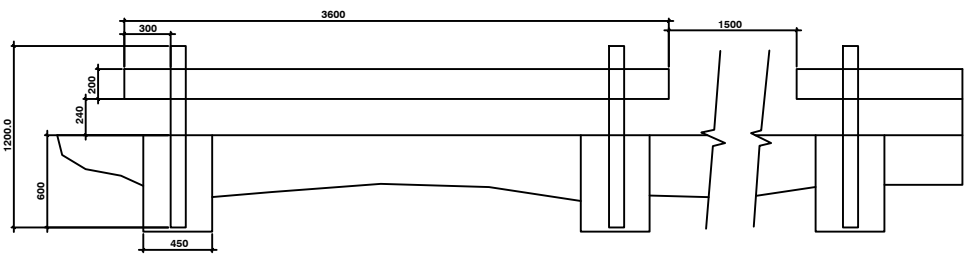
Low vehicle exclusion fence / bollard
